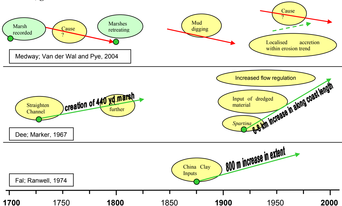
Figure 2. Conceptual drawing illustrating effects of some human activities (in addition to/other than land reclamation) on different saltmarshes. Slope of the arrow is indicative of the rate of accretion and/or erosion. Red arrows indicate erosion, green indicate accretion.
