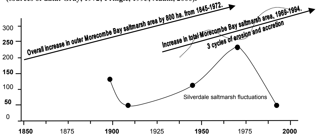
Figure 1. Conceptualised drawing of accretion and erosion cycles of Silverdale Marsh compared with the saltmarshes of the entire Morecombe Bay area (sources of data: Gray, 1972; Pringle, 1995; Adam, 2000).
