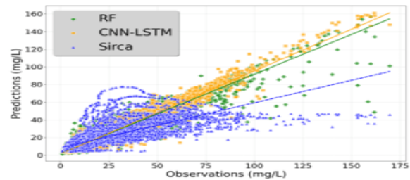
Fig. 1: Comparison of models: Saône river case
